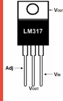
Lm317t Integrated Circuits
